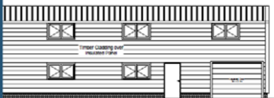
Front Elevation
